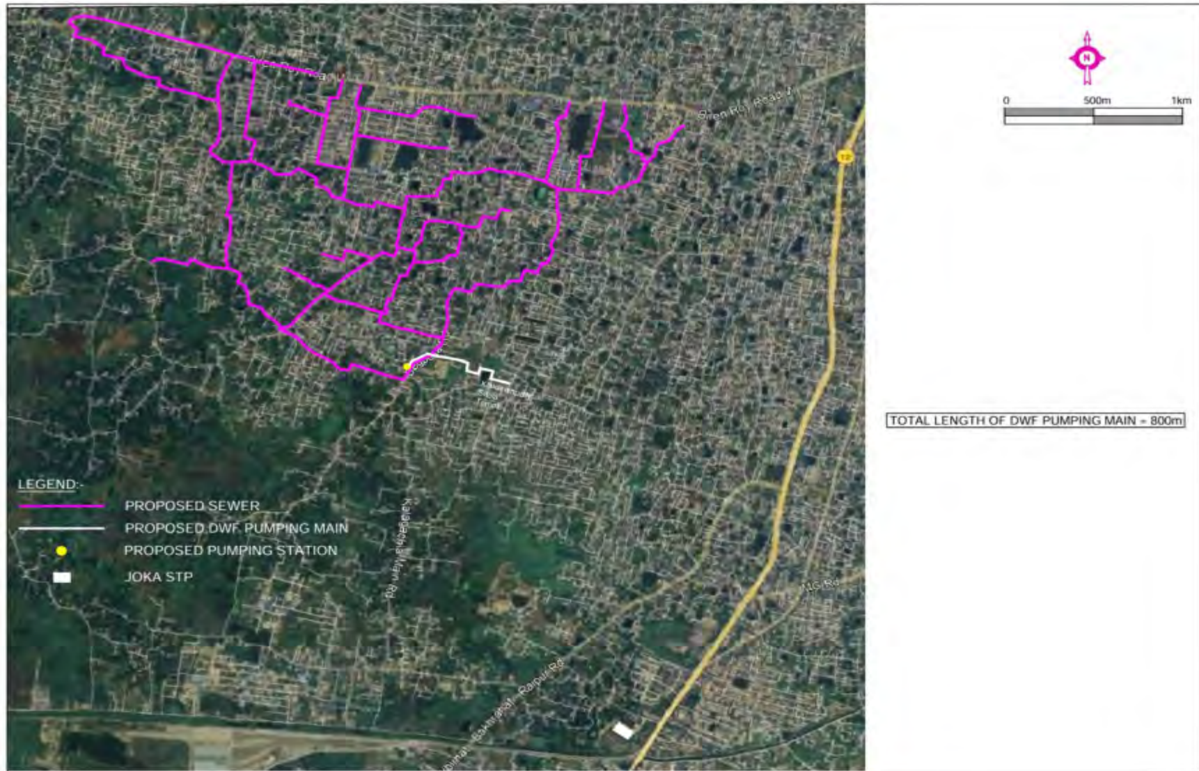
Figure 12: DWF Pumping Main from proposed Keyatala Pumping Station
