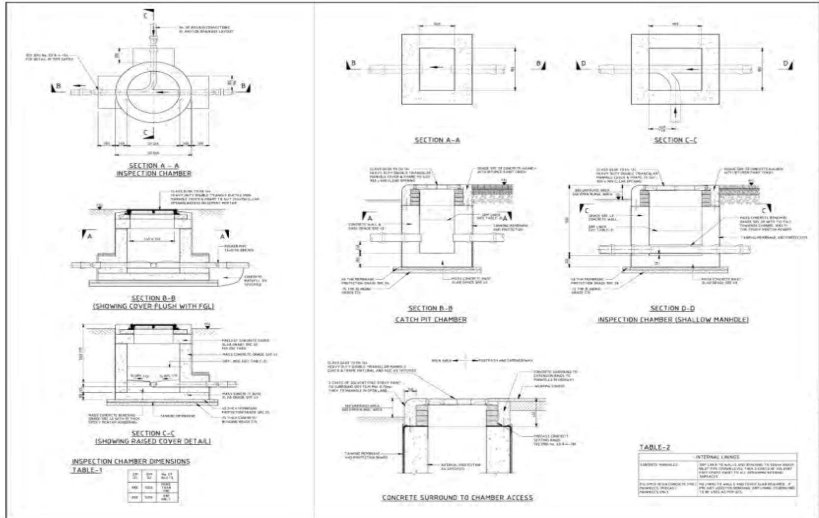
Figure 15: Typical Design of Catch Pit, Gully Pit, and Inspection Pit
