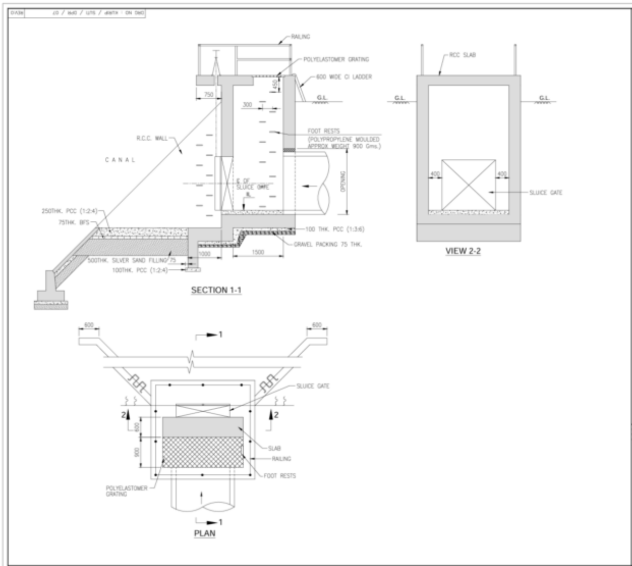
Figure 16: Typical outfall structures for Sluice Gate
