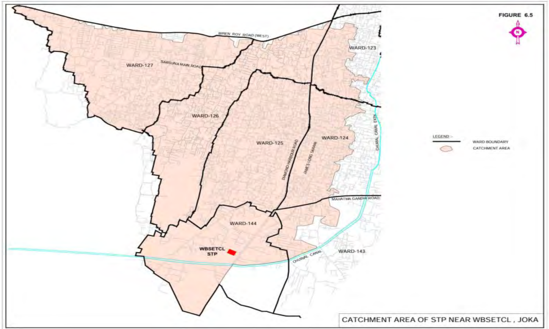
Figure 14: Catchment Area of Bank plot STP (Under KEIIP Trench 3)
