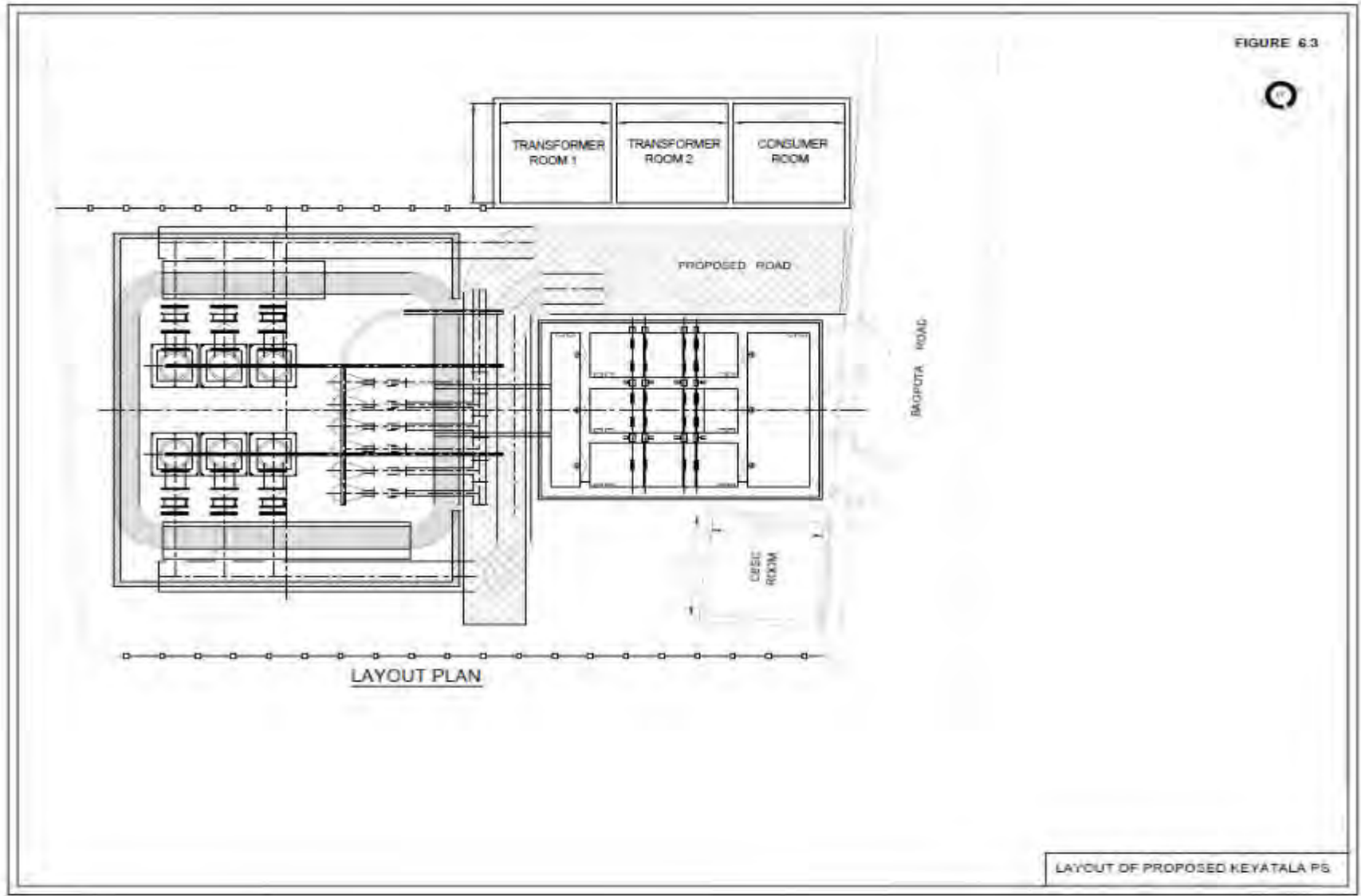
Figure 10: Proposed Pumping station Layout at Keyatala (SD 09) (Note: this layout plan is only tentative)
