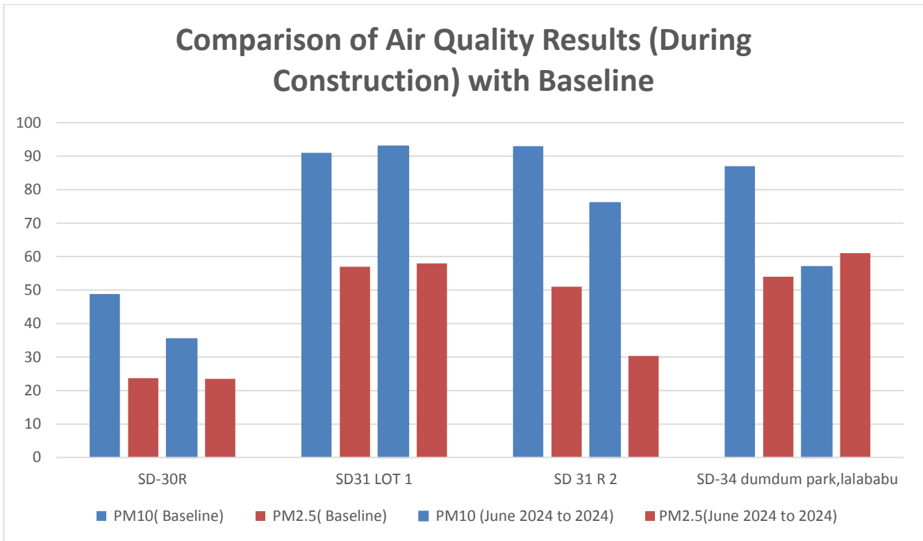
Figure 5: Comparison of During Construction Monitoring Results with Baseline
